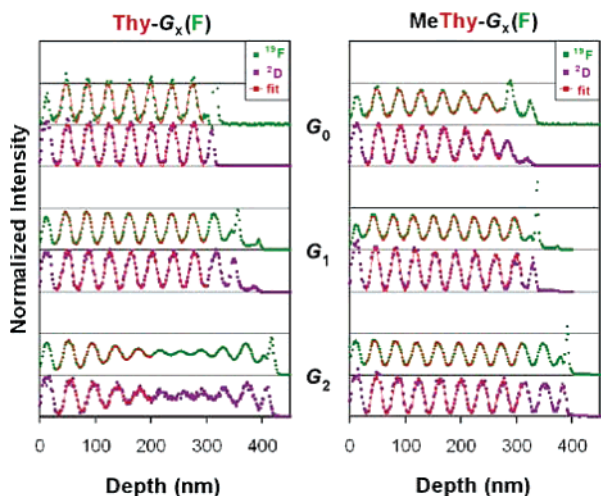
Figure 5. SIMS traces of the ^{19}\text{F} (green) and ^2\text{D} (purple) signals of thin films of the PS- b -dPS/DAP polymer with the Thy- G_x (F) and MeThy- G_x (F) molecules (at 0.9 DAP-equivalents). All traces were normalized to obtain the same offset of their sinusoidal wave and shifted vertically for clarity.
